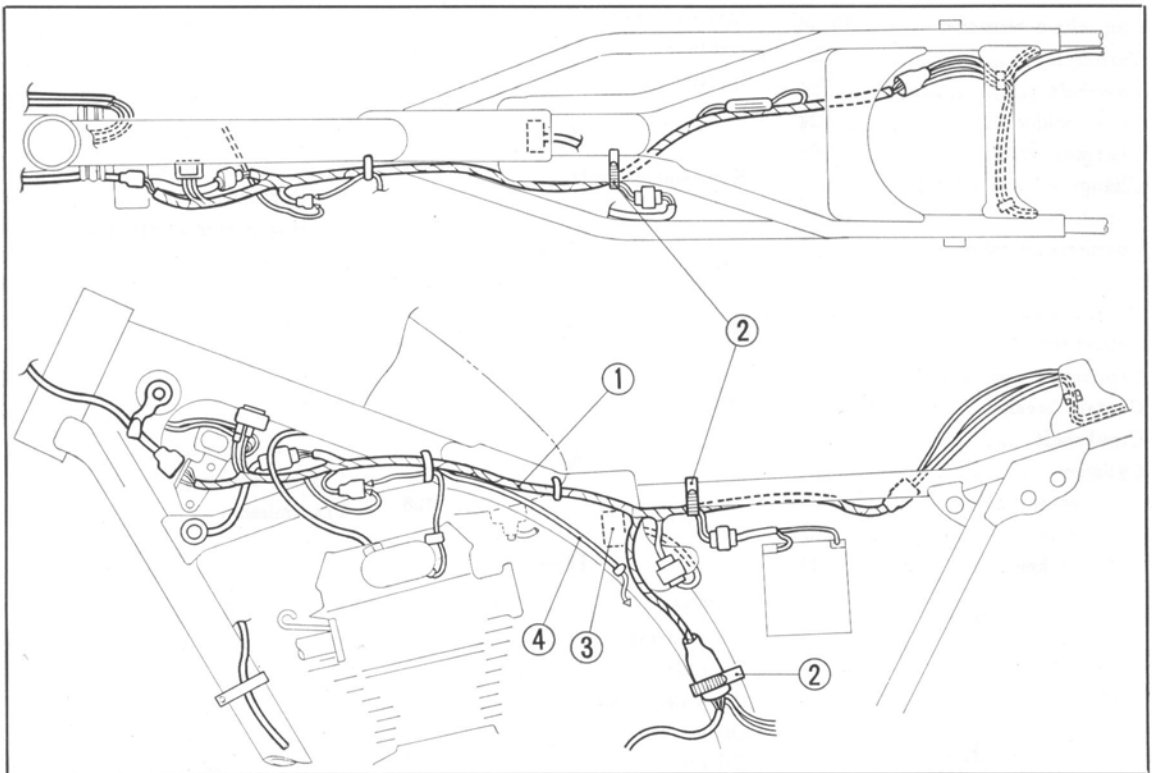
① Wire harness assy ② Wire harness band ③ Siricon rectifier ④ Throttle cable
